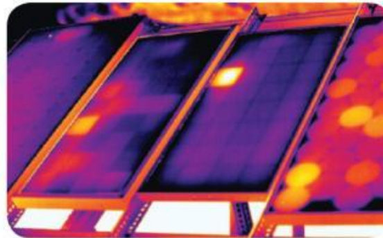
Figure 3. Solar cell testing using an uncooled microbolometer handheld camera.
